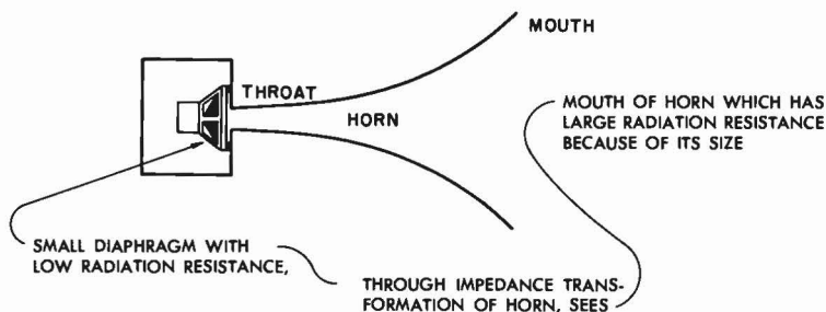
Fig. 10-3. Small diaphragm is better match to "all the air" through the horn as an impedance transformer.
