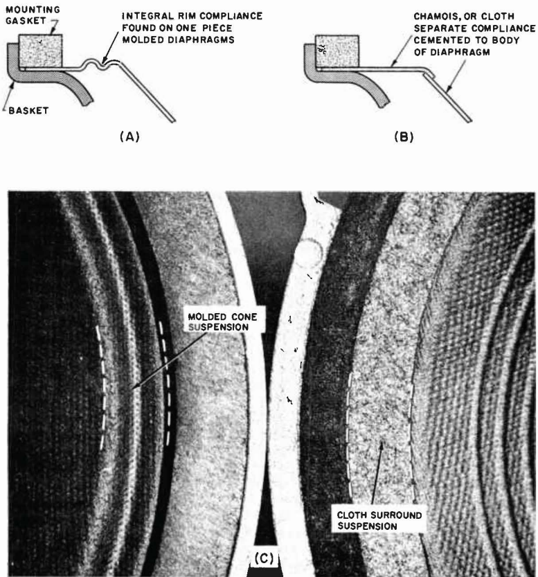
Fig. 2-10. Forms of diaphragm suspension.
