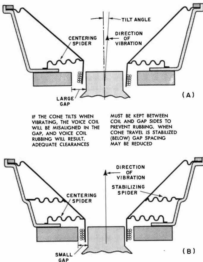
Fig. 4-7. Where mechanical vibration is precisely controlled, greater magnetic gap efficiency may be obtained.
