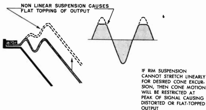
Fig. 4-5. For clean peak signal reproduction, edge suspension must have mechanically linear motion for full diaphragm excursion.
