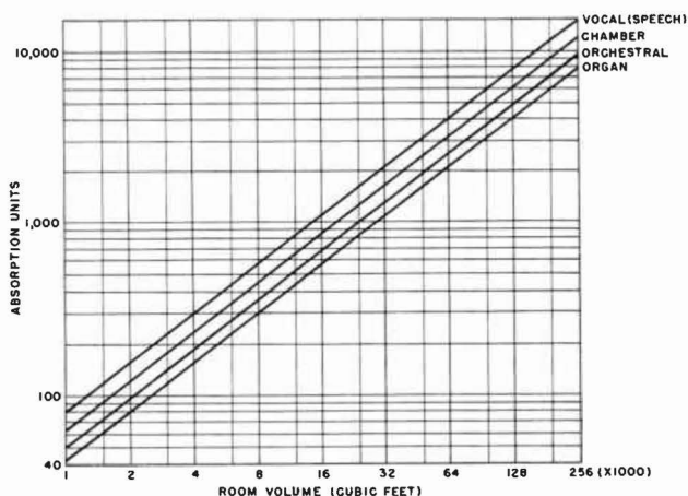
Fig. 17-3. Total absorption units required for a given room volume for different types of program material.
