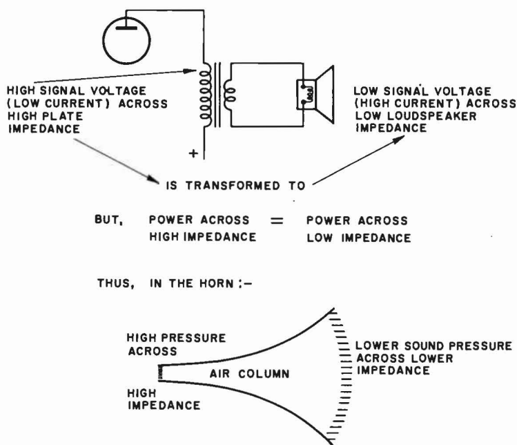
Fig. 10-2. Analogy showing the impedance transformation function of a horn.
