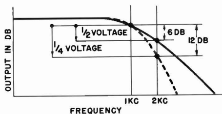
Fig. 7-11. When voltage drops to \frac{1}{2} the value of the voltage at the crossover frequency, the attenuation is 6 db; if it drops to \frac{1}{4} , the attenuation is 12 db. If this drop takes place in a span of one octave, there is either a 6 or a 12 db per octave attenuation.
