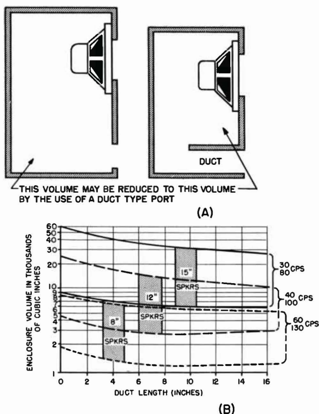
Fig. 9-13. Reduction in size of enclosure that may be realized through use of a duct, which creates a larger port inductance, permitting smaller cavity capacitance.
