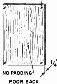
Fig. 14-1. The back of the bass-reflex cabinet will cause waveform deterioration and loss of level at low frequencies if it is weak and poorly mounted.
