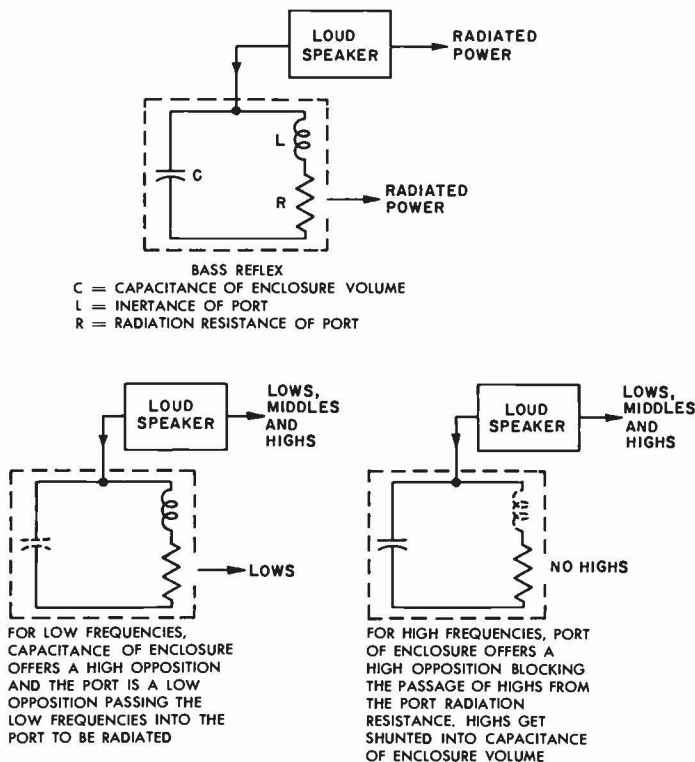
Fig. 13-1. The capacitance of the bass-reflex enclosure and the inductance of its port act as L-C elements of a crossover network, allowing lows from the port and restricting middles and highs to the speaker.
