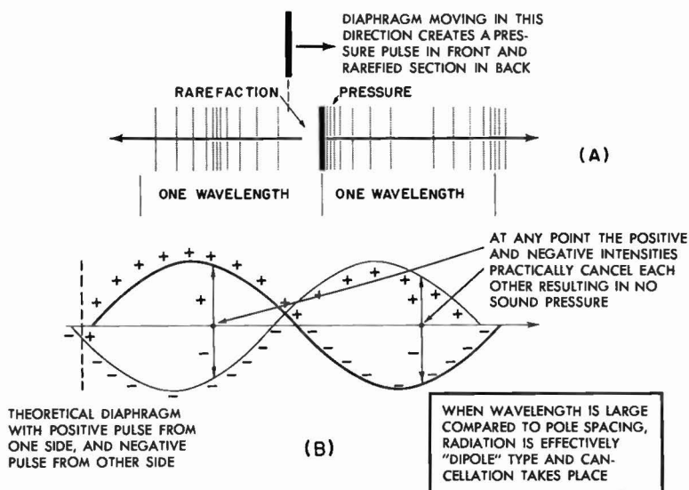
Fig. 9-2. Doublet operation of un baffled diaphragm.
