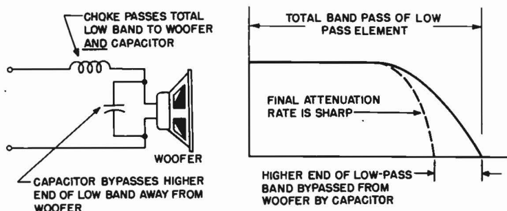
Fig. 7-7. A sharp cutoff low-pass filter is made by shunting a high-pass element across the woofer circuit.
