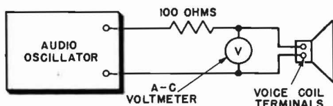
Fig. 9-11. Apparatus for determining the resonant frequency of a loudspeaker. At the resonant frequency the voltmeter will read maximum.
