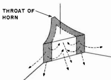
Fig. 16-4. The split folded horn couples into the corner of the room through two mouths, with the horn sections effectively removed behind the corner.
