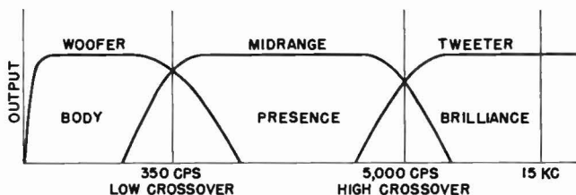
Fig. 6-10. A three-way multi-speaker system comprising components selected by the manufacturer on the basis of compatible efficiencies, overlapping areas, and angular dispersion, with matched network. System uses wide angle reciprocating flare horns and crossovers at 350 and 5000 cps. (Courtesy University)
