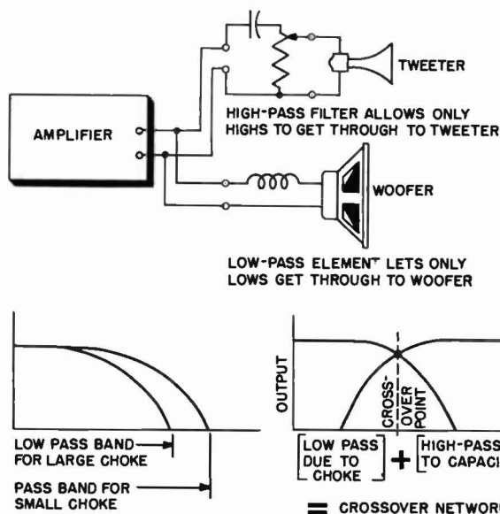
Fig. 7-3. Low-pass filter plus high-pass filter form a crossover network. (Network shown has a 6 db per octave attenuation.)
