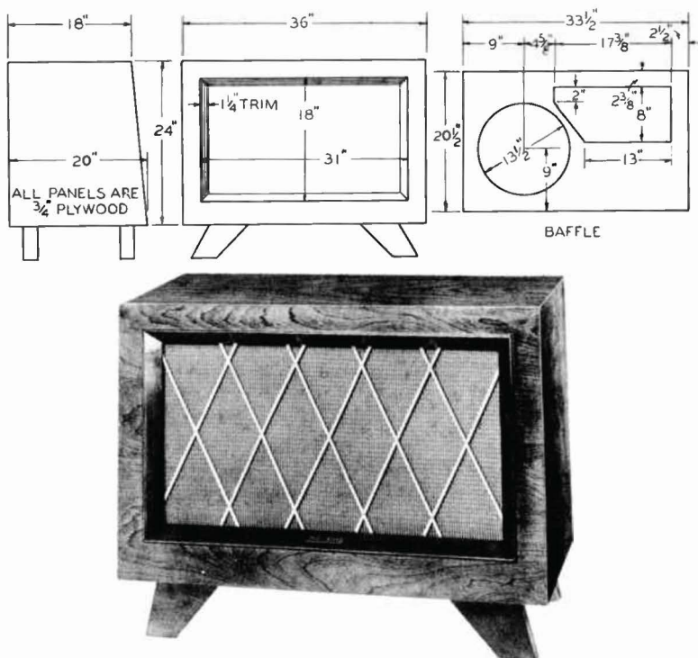
Fig. A-16. Wall type bass reflex (Stephens Low-Boy, Model 610).
