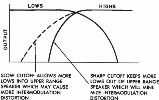
Fig. 7-13. The sharpness of the attenuation rate of the system will determine the degree of intermodulation distortion which may occur if the speakers are not perfectly linear.
