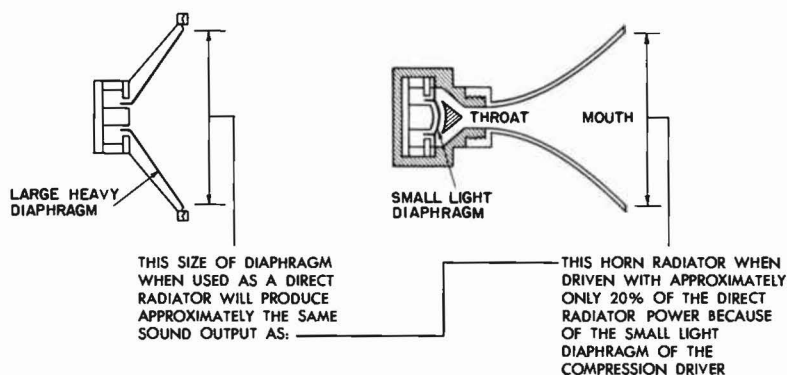
Fig. 3-13. The compression type driver has a small, light diaphragm, which is easier to drive than a large cone diaphragm. The pulsations produced by the diaphragm at the narrow throat are transmitted to the horn mouth, which becomes the radiating surface.
