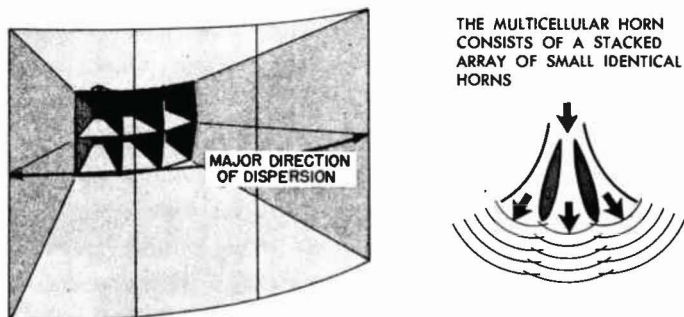
Fig. 3-16. The multicellular horn field pattern is made of separate sound beams radiated by small individual horns arranged in an arc.
