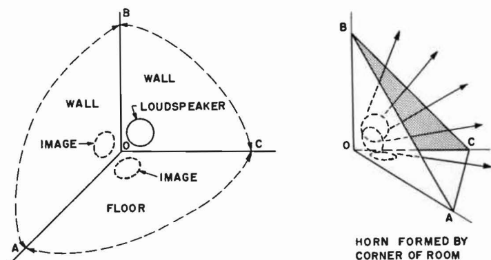
Fig. 16-2. When the speaker is placed down in the corner, two acoustic images are formed on the wall and floor. These multiple sound sources, located in the corner, act as a single larger radiator at the apex of a three sided horn.
