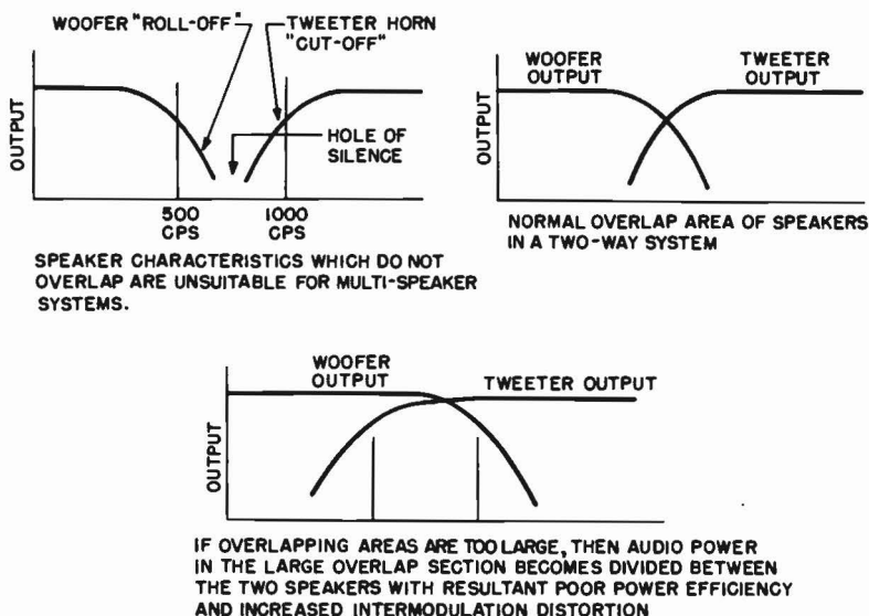
Fig. 6-4. For maximum smoothness of response, speakers should have compatible roll-off and cutoff slopes.
