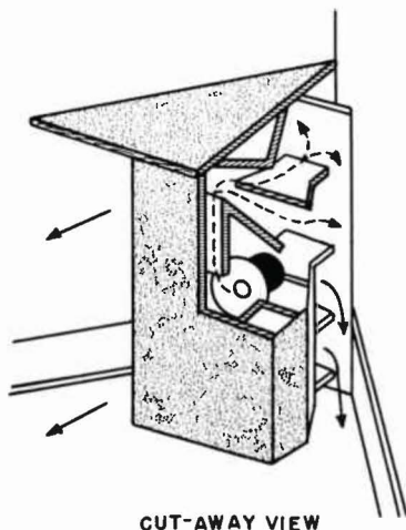
Fig. 8-5. The folded horn may be designed to be completely corner loaded by the walls of the corner of the room. (Klipschorn)
