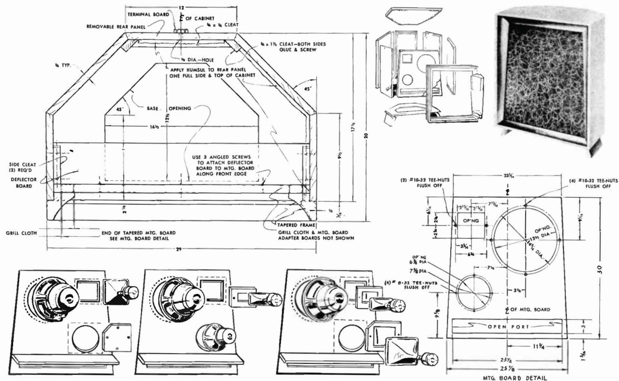
Fig. A-12. Cornerless corner horn loaded port bass reflex (University EN-15).
