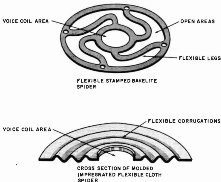
Fig. 2-8. Some typical voice coil centering devices (spiders).
