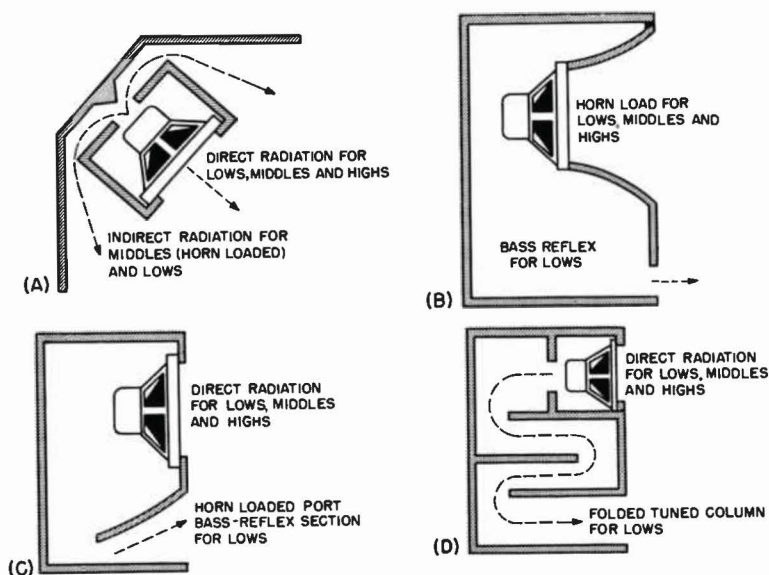
Fig. 8-3. Combinations of direct and indirect radiators.
