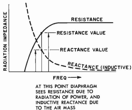
Fig. 10-11. Another effect of the compression chamber is to make the load seen by the diaphragm more resistive by balancing the air mass inertance with the chamber stiffness reactance.
