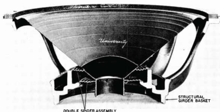
Fig. 4-9. Girder basket construction and double spider construction ensure minimum basket deformation and precision voice coil alignment. (Courtesy Audio Engineering Society, July 1954, "Mechanics of Good Loudspeaker Design")
