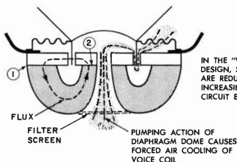
Fig. 4-8. Magnetic circuit efficiencies may be increased by reducing number of surfaces.
