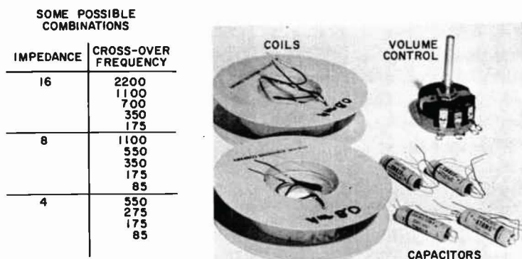
Fig. 7-14. Network kit that may be obtained for constructing network. Individual coils or kits are available for the above tabulated requirements. (Courtesy General Apparatus)
